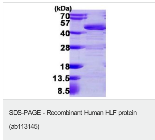
15% SDS-PAGE analysis of ab113145 (3µg)
