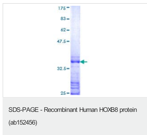
12.5% SDS-PAGE gel showing ab152456 stained with Coomassie Blue
