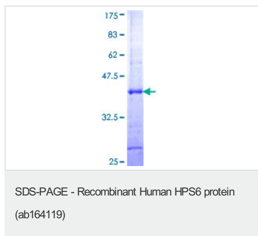
ab164119 on a 12.5% SDS-PAGE stained with Coomassie Blue.
