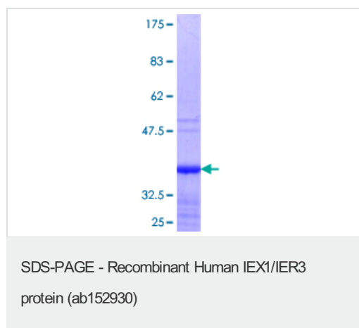
ab152930 on a 12.5% SDS-PAGE stained with Coomassie Blue.
