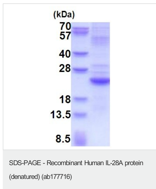
15% SDS-PAGE analysis of ab177716 (3µg).
