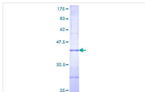
ab160204 on a 12.5% SDS-PAGE stained with Coomassie Blue.
