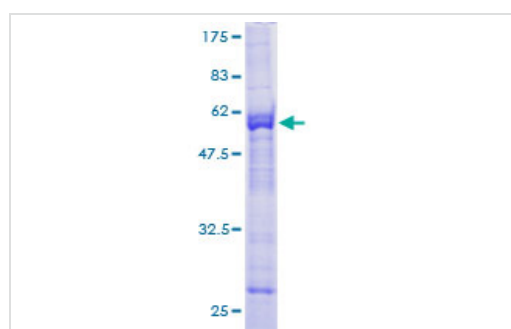
SDS-PAGE - Recombinant Human KLHDC3 protein (ab165097)
