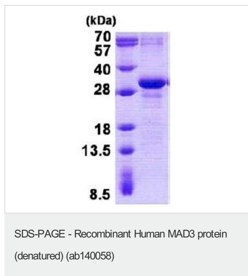
15% SDS-PAGE analysis of ab140058 (3µg)
