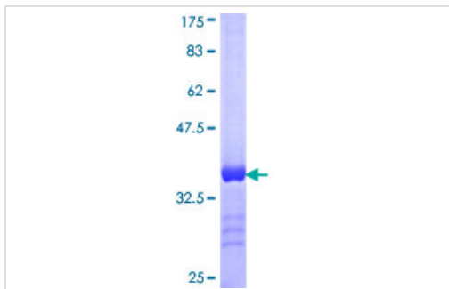
ab166430 on a 12.5% SDS-PAGE stained with Coomassie Blue.
