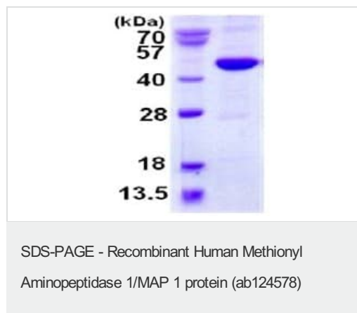
15% SDS-PAGE showing ab124578 (3µg).
