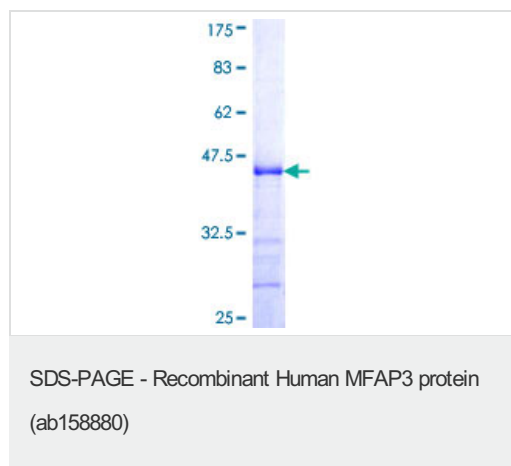
ab158880 on a 12.5% SDS-PAGE stained with Coomassie Blue.
