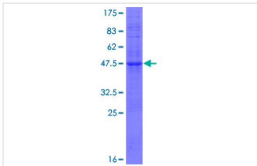
ab166579 on a 12.5% SDS-PAGE stained with Coomassie Blue.
