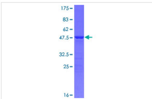
ab163693 on a 12.5% SDS-PAGE stained with Coomassie Blue.
