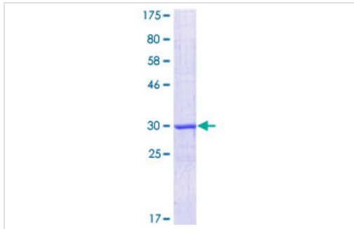
SDS-PAGE - Recombinant Human MKRN3 protein (ab159863)
