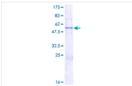
ab162825 on a 12.5% SDS-PAGE stained with Coomassie Blue.
