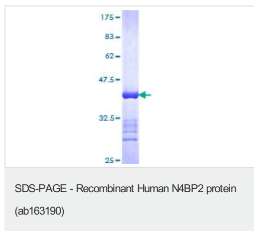
ab163190 on a 12.5% SDS-PAGE stained with Coomassie Blue.
