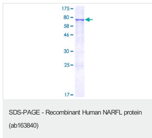
ab163840 on a 12.5% SDS-PAGE stained with Coomassie Blue.
