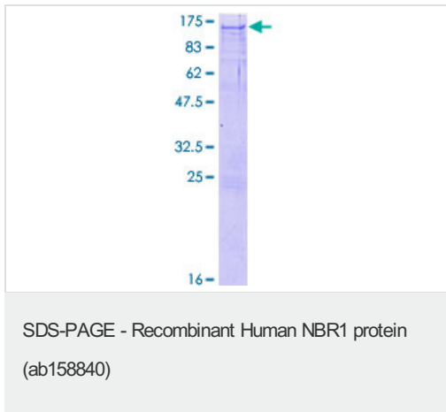
ab158840 on a 12.5% SDS-PAGE stained with Coomassie Blue.
