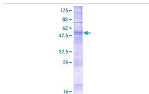
12.5% SDS-PAGE analysis of ab152721 stained with Coomassie Blue.
