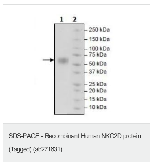
SDS-PAGE analysis of ab271631.
