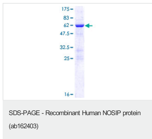
ab162403 on a 12.5% SDS-PAGE stained with Coomassie Blue.
