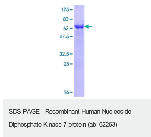
ab162263 on a 12.5% SDS-PAGE stained with Coomassie Blue.
