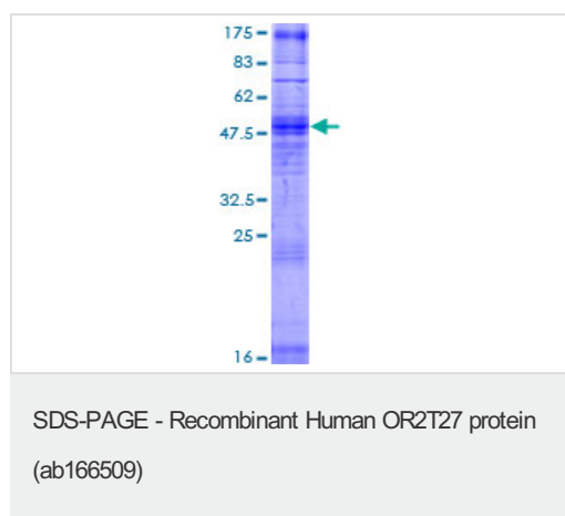
ab166509 on a 12.5% SDS-PAGE stained with Coomassie Blue.
