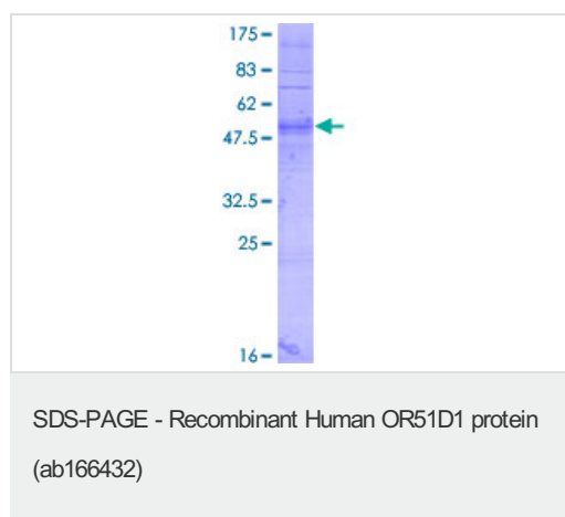
ab166432 on a 12.5% SDS-PAGE stained with Coomassie Blue.
