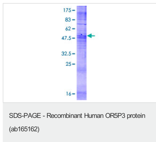
ab165162 on a 12.5% SDS-PAGE stained with Coomassie Blue.
