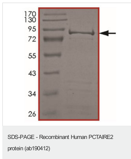
SDS-PAGE analysis of ab190412
