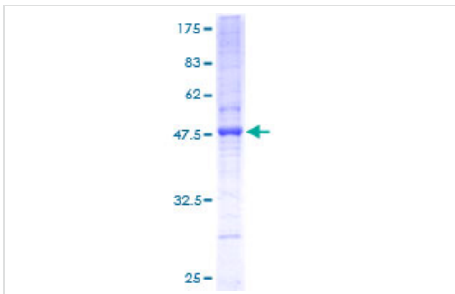
SDS-PAGE - Recombinant Human PIGH protein (ab159122)
