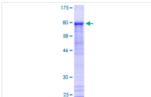
ab163746 on a 12.5% SDS-PAGE stained with Coomassie Blue.
