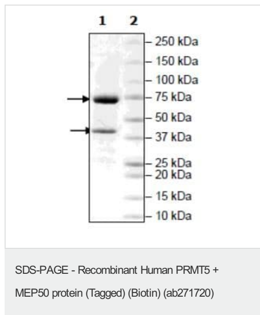
SDS-PAGE analysis of 4 µg ab271720.
