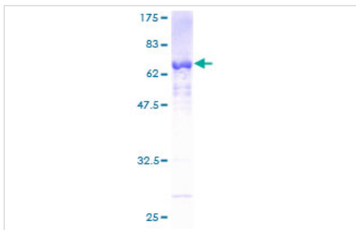
ab160099 on a 12.5% SDS-PAGE stained with Coomassie Blue.
