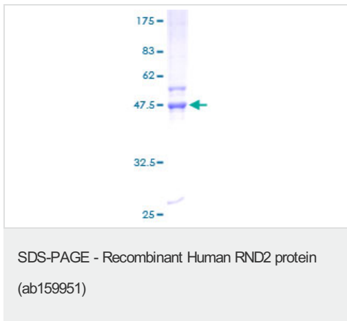
ab159951 on a 12.5% SDS-PAGE stained with Coomassie Blue.
