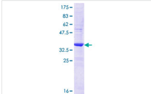
ab163477 on a 12.5% SDS-PAGE stained with Coomassie Blue.
