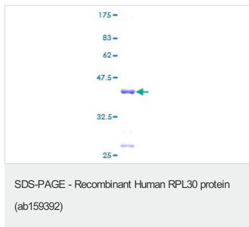
ab159392 on a 12.5% SDS-PAGE stained with Coomassie Blue.
