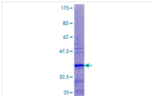
ab159405 on a 12.5% SDS-PAGE stained with Coomassie Blue.
