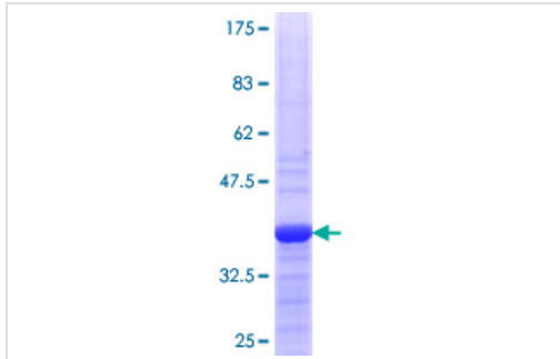
SDS-PAGE - Recombinant Human RPS8 protein (ab159434)
