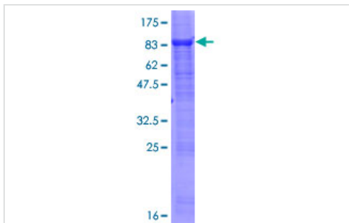
ab153542 on a 12.5% SDS-PAGE stained with Coomassie Blue.
