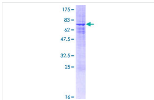
ab161600 on a 12.5% SDS-PAGE stained with Coomassie Blue.
