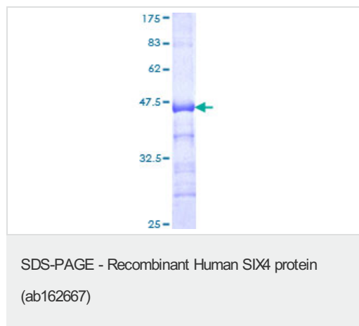
ab162667 on a 12.5% SDS-PAGE stained with Coomassie Blue.
