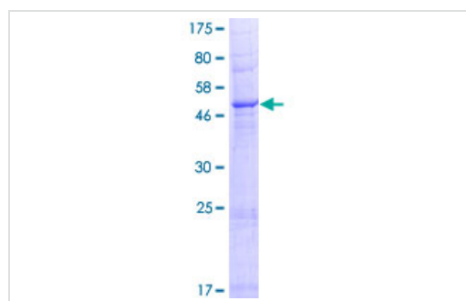
SDS-PAGE - Recombinant Human SLC35A4 protein (ab165011)
