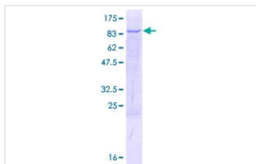
12.5% SDS-PAGE analysis of ab132734 stained with Coomassie Blue.
