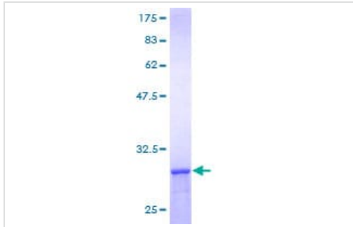
ab161115 on a 12.5% SDS-PAGE stained with Coomassie Blue.
