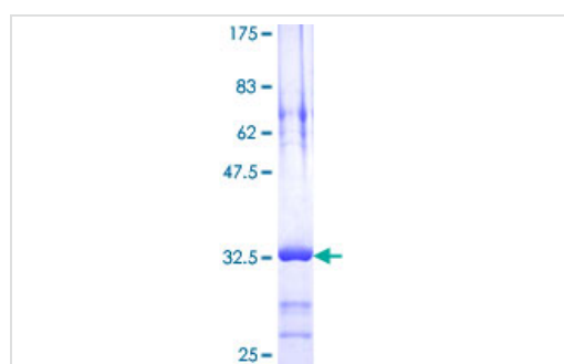
12.5% SDS-PAGE showing ab112365 at approximately 30.84 kDa, stained with Coomassie Blue.
