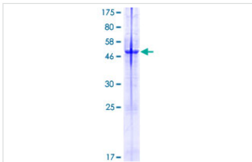
ab164454 on a 12.5% SDS-PAGE stained with Coomassie Blue.
