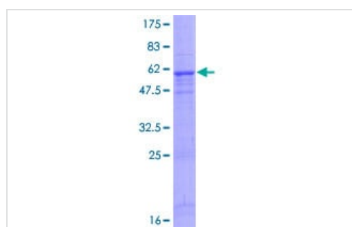
12.5% SDS-PAGE analysis of ab132329 stained with Coomassie Blue.
