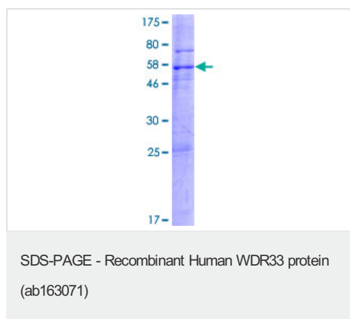
ab163071 on a 12.5% SDS-PAGE stained with Coomassie Blue.
