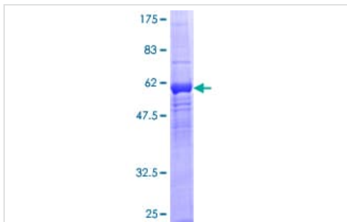
ab162780 on a 12.5% SDS-PAGE stained with Coomassie Blue.
