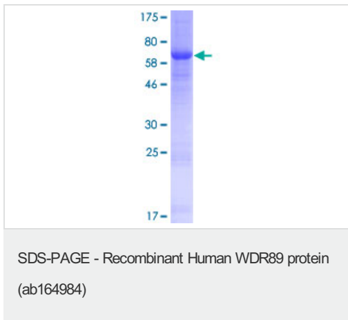
ab164984 on a 12.5% SDS-PAGE stained with Coomassie Blue.
