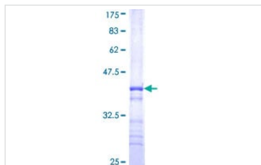
ab163264 on a 12.5% SDS-PAGE stained with Coomassie Blue.
