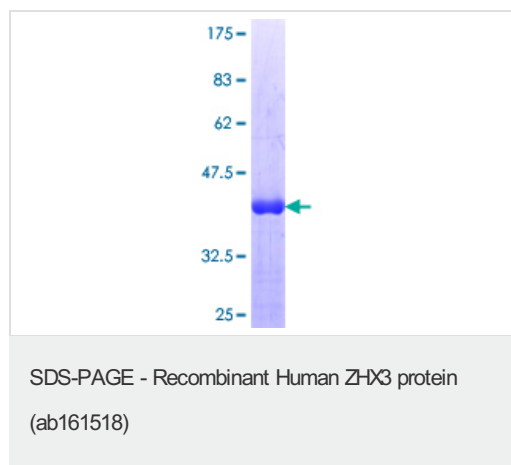
ab161518 on a 12.5% SDS-PAGE stained with Coomassie Blue.
