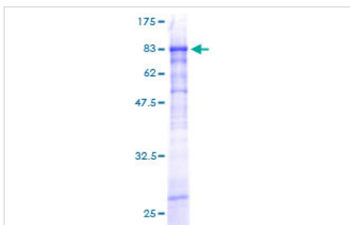
ab159839 on a 12.5% SDS-PAGE stained with Coomassie Blue.
